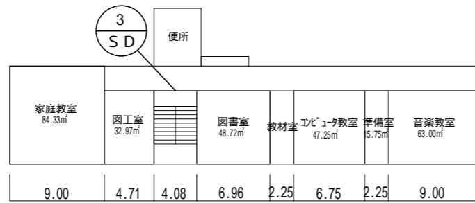
⑧ 3階
