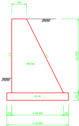
SGW42 S=1:20
