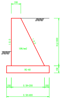
SGW17 S=1:20
