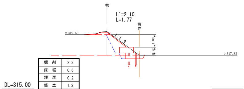
SECT 0.0 GH=319.86
